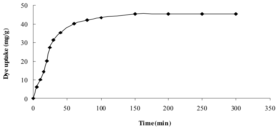
Fig. 5. Effect of contact time on sorption of MG dyes by the Hydrilla Verticillata biomass - initial dye concentration: 100 mg/L, sorbent mass: 0.55 g; agitation speed: 200 rpm)
