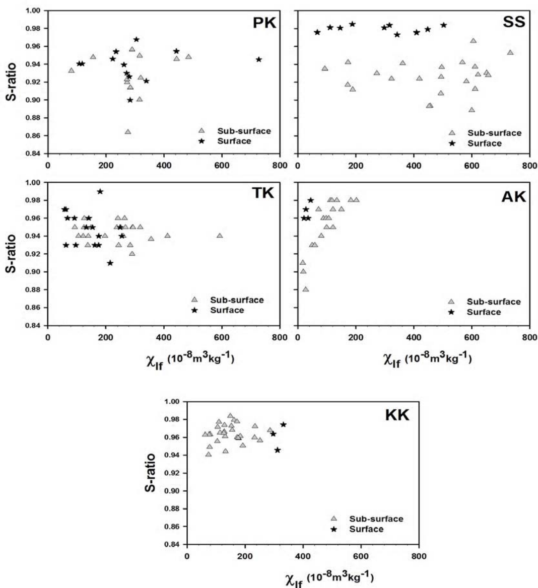
Fig. 12. S-ratio vs. \chi_{lf} for soil samples from the catchments of Pookot Lake; Shantisagara; Thimmanayanakanakere; Ayyannakere; and Kurburkere. Samples from PK, TK, AK and KK do not have profound differences in their magnetic mineralogy. In SS, the magnetic mineralogy is distinct, with the surface soil samples having a soft magnetic mineralogy (S-ratio > 0.96), and the sub-surface ones having a relatively higher contribution from hard magnetic minerals
