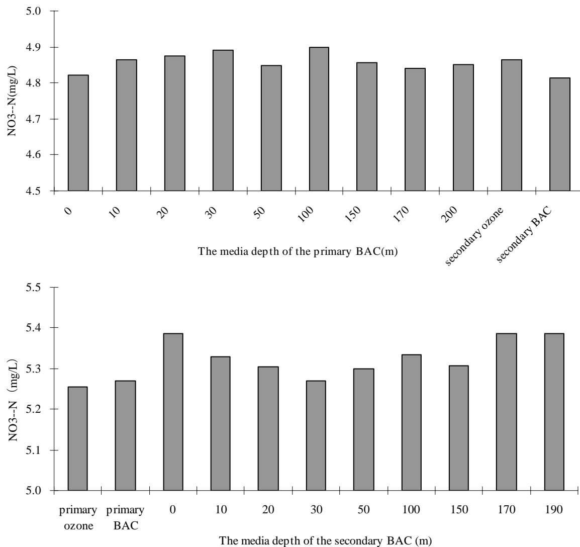
Fig. 4. \text{NO}_3\text{--N} variations along the depth of each stage of BAC
