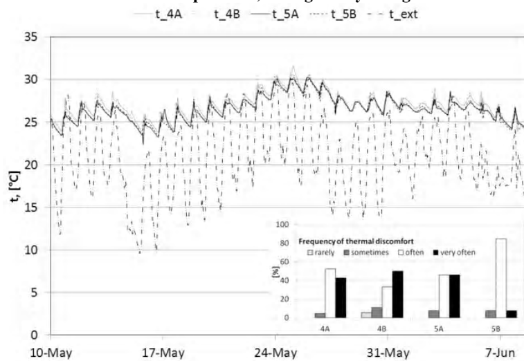
Fig.4. Frequency of pupils' thermal comfort related to air temperature profiles
