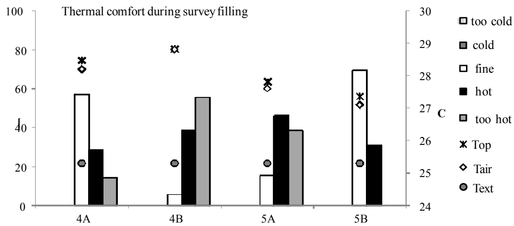
Fig. 3. Pupils' thermal sensation, related to measured operative and air indoor temperature and external temperature, during survey filling
