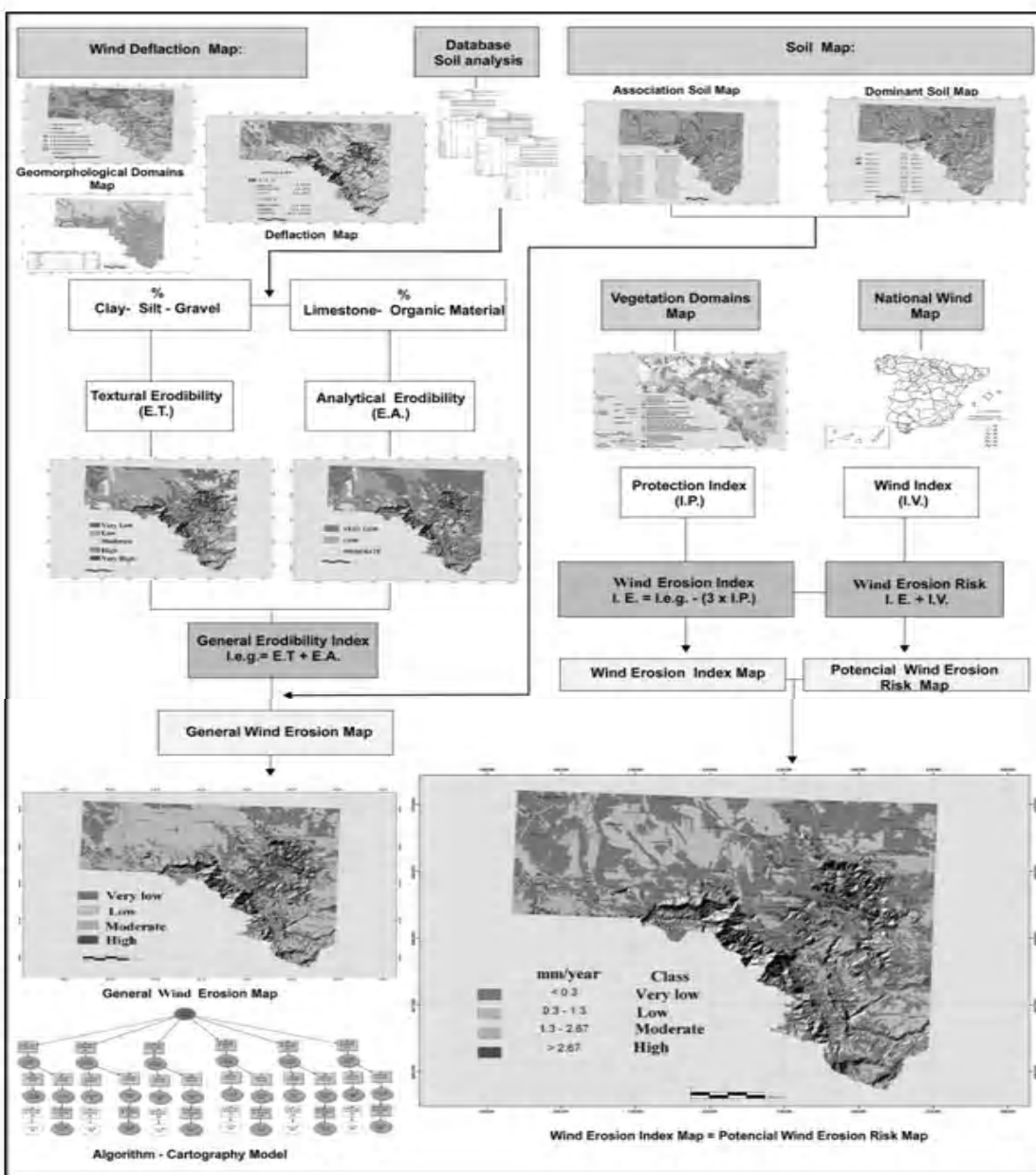
Fig. 4. Schematic of the procedure for calculation of wind erosion
