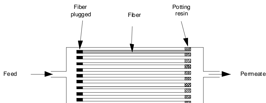
Fig. 1. shows the scheme of a hollow-fiber module operating in outside-in and dead-end mode
