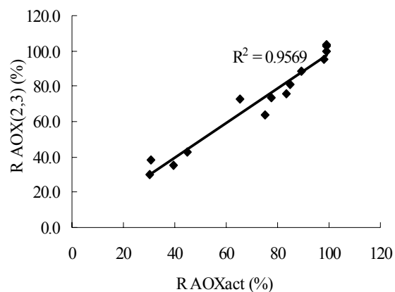
Fig. 3. Predicted vs. actual of AOX removal efficiencies for equations 2 and 3
