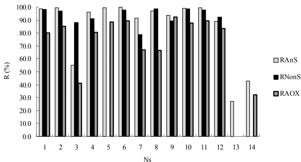
Fig. 2. Removal efficiencies of surfactants ( R_{AnS} and R_{NonS} ) and AOX ( R_{AOX} )
