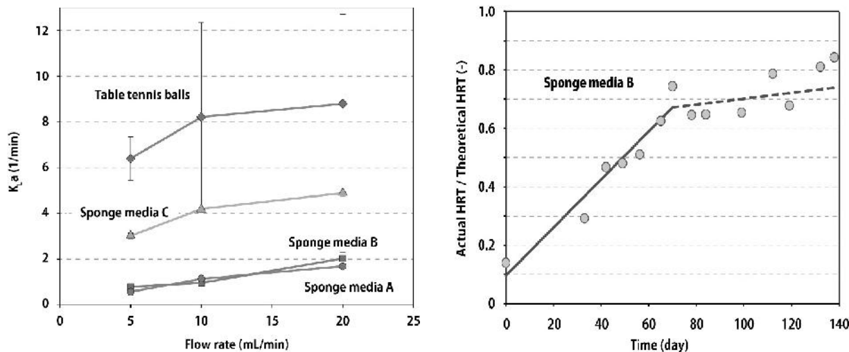
Fig. 8. Changes of K_La with flow rate
