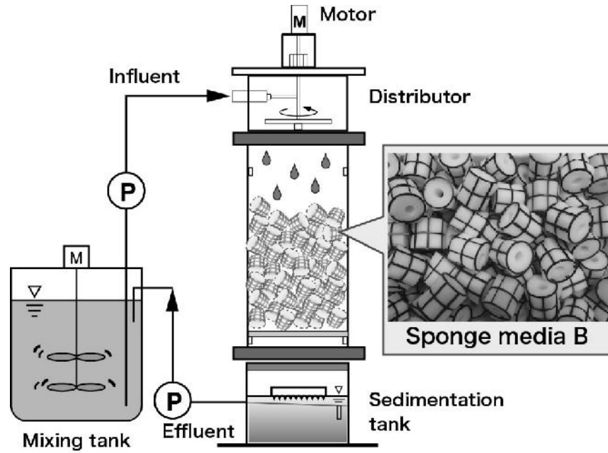
Fig. 4. Experimental packed sponge setup
