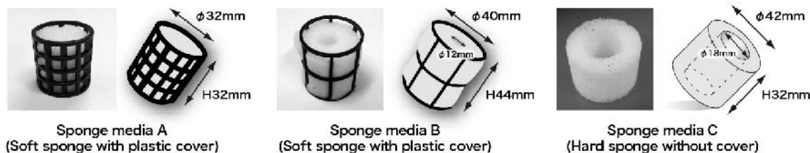
Fig. 2. Sponge support media used in this study
