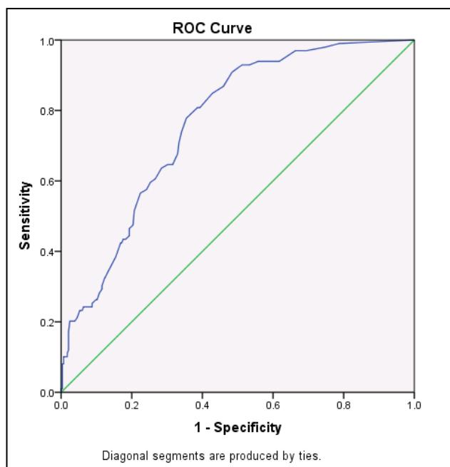
Figure 1. ROC Curve of SOMS-7 Questionnaire for Anxiety/Mood Disorder Patients
