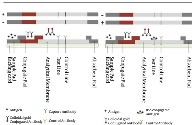
Figure 2. Two Formats of Lateral Flow Immunoassay
