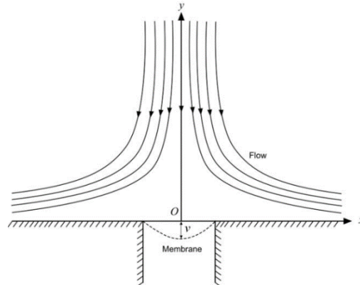
Fig. 1. Two dimensional stagnation point flow near the membrane.
