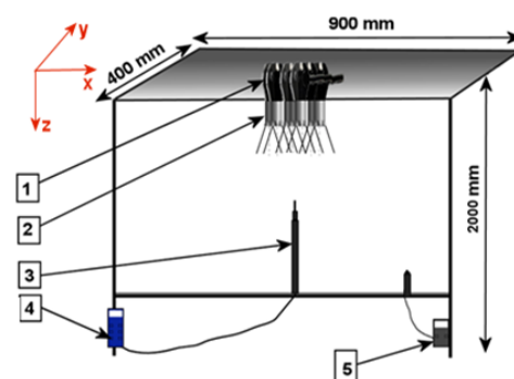
1- Hair dryer; 2- Lobed nozzles; 3- Thermo-anemometer probe; 4- Thermo-anemometer; 5- Thermometre Fig. 1. Schematic diagram of experimental setup.
