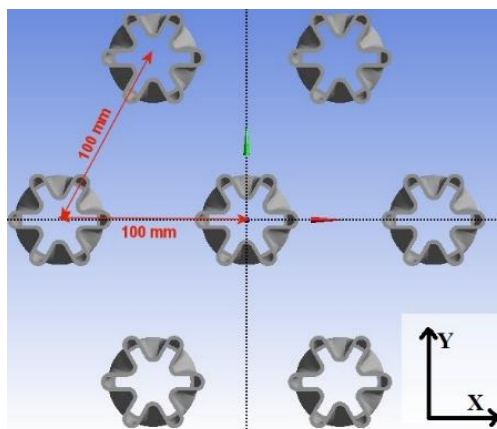
Fig. 3. Multiple lobed jet configuration.
