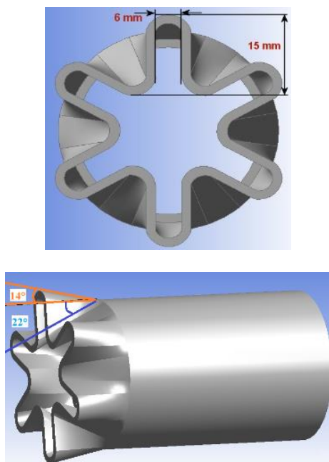
Fig. 2. Geometry of lobed diffusers.
