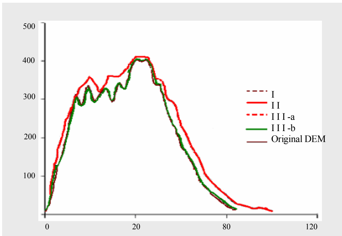
Figure 9- Slop frequency distribution.
