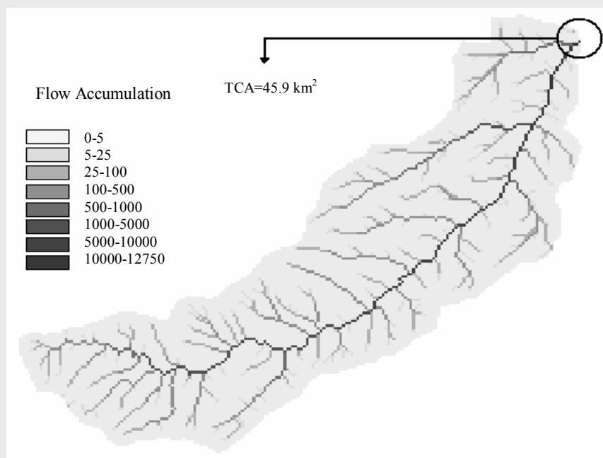
Figure 5- Flow accumulation map for algorithm IIIa.
