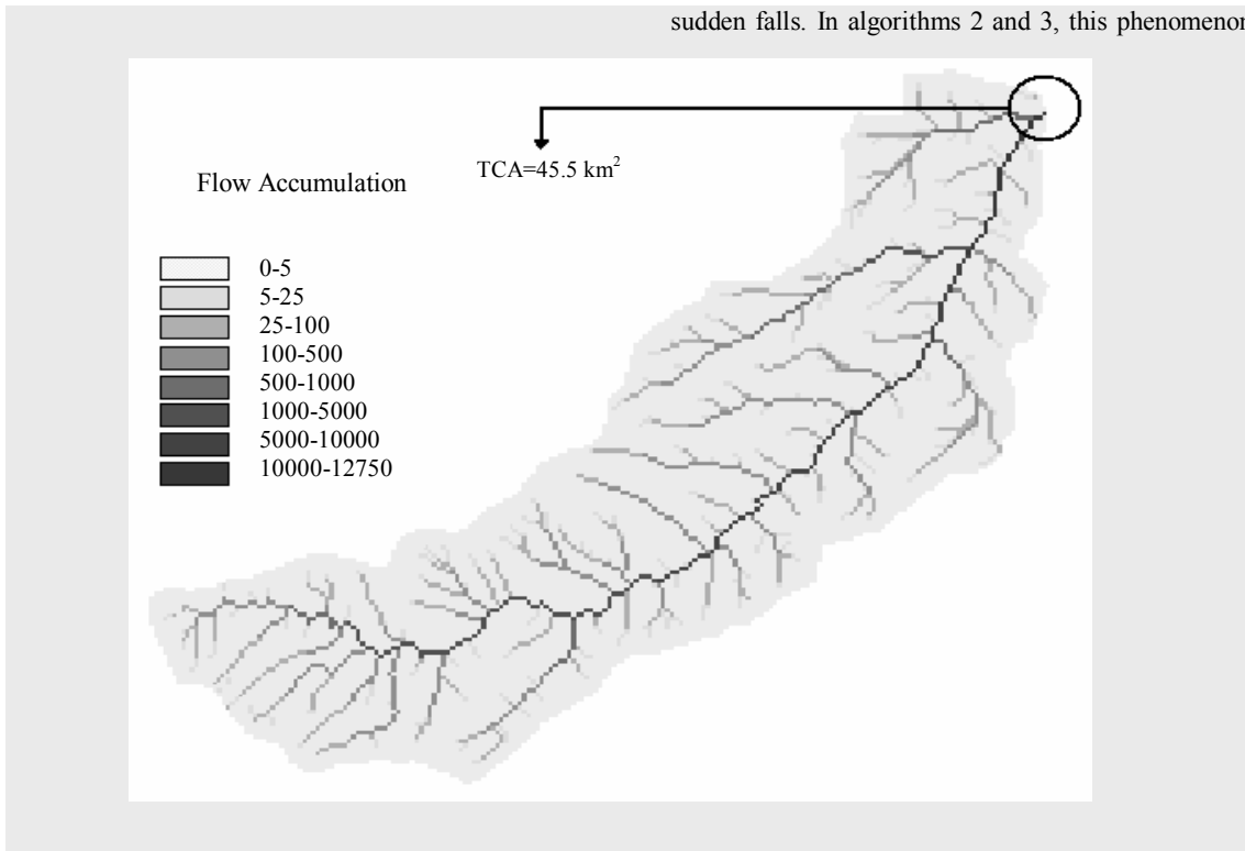
Figure 6- Flow accumulation map of algorithm IIIb.
