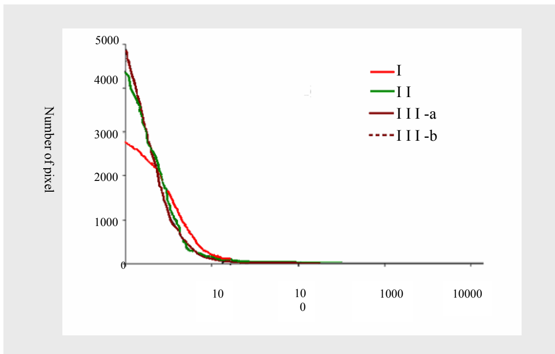
Figure 8- Flow accumulation frequency distribution.
