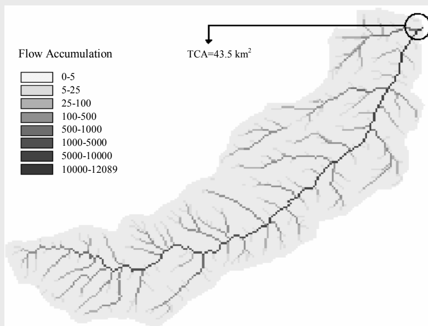
Figure 4- Flow accumulation map for algorithm II.
