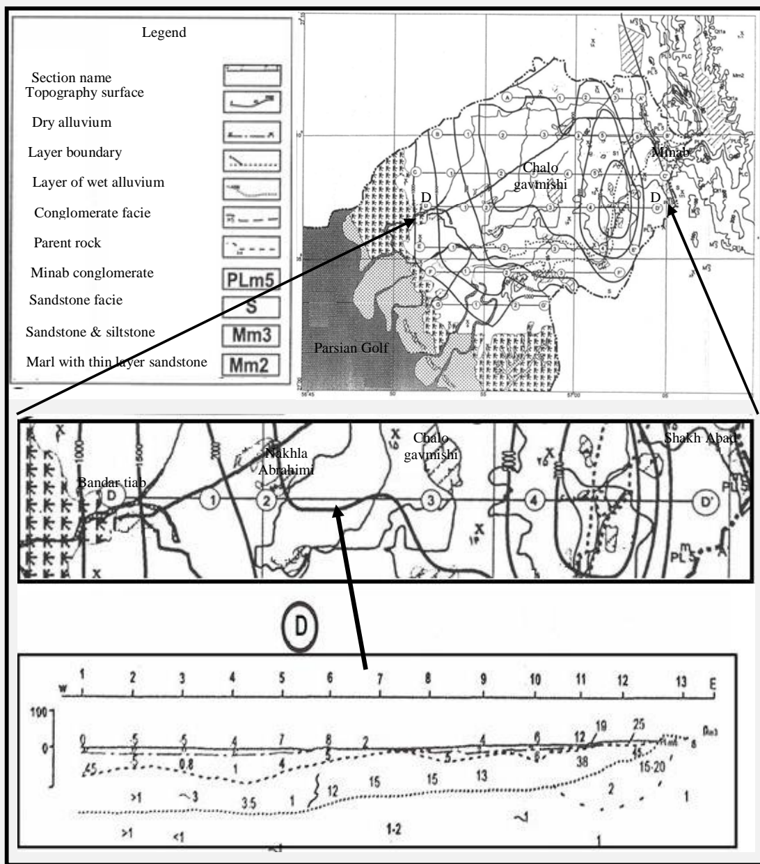
Figure 6. Geological cross section using the geoelectric method.
