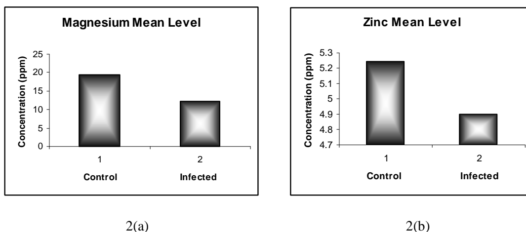
Fig. 2: (a) The reduced magnesium means level result of control and malarial patients while figure 2(b) Decreased zinc mean level result of control and malarial patients
