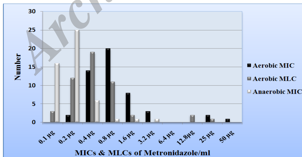
Fig .1: Comparison of metronidazole MICs and MLCs of Iranian T. vaginalis isolates under both aerobic and anaerobic environments
