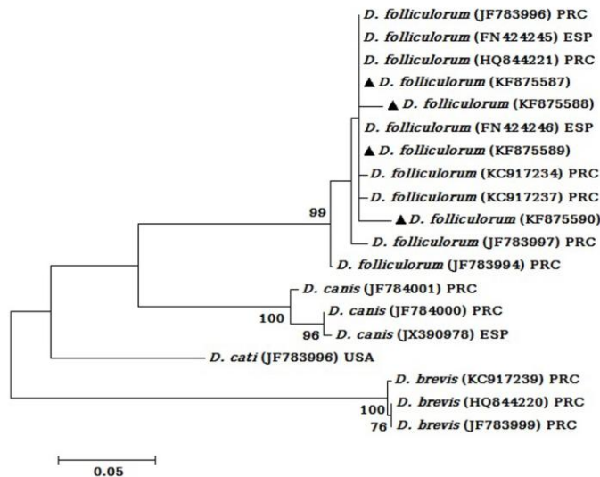
Fig. 1: Phylogenetic tree of the mitochondrial 16S ribosomal DNA nucleotide sequences of D. folliculorum . The tree was constructed by using the Maximum-Likelihood test and Tamura-3 parameter model in MEGA software version 6. The numbers above the branches indicate the percentage of bootstrap samplings percentages. Branches without numbers have frequencies of less than 75%. Besides the isolates reported in this study, which are marked by a black filled triangle, some accession numbers from other studies were applied in phylogenetic analysis. Abbreviations: PRC: People’s Republic of China; USA: United States of America; ESP: Spain
