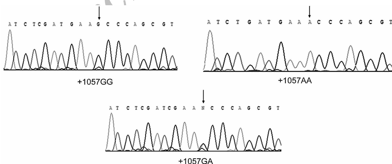
Figure 1. Sequence profiles of CD86 +1057GA genotypes.
