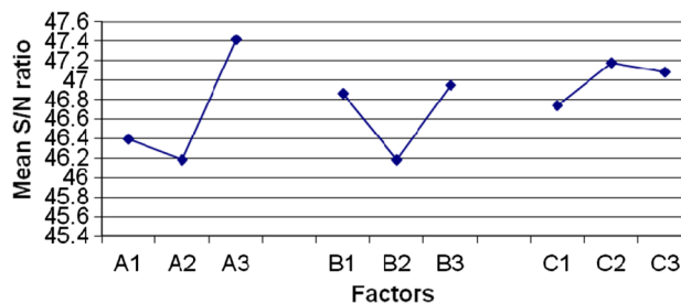
Fig. 2 S/N graph showing readability performance for factors A, B and C (15° viewing angle)
