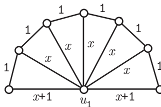
FIGURE 5. One possible magic labeling of F_8 .
