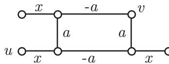
FIGURE 1. An example of a non-magic graph.
