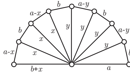
FIGURE 6. A typical magic labeling of F_{10} .
