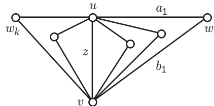
FIGURE 13. A typical labeling of B(3, k) .
