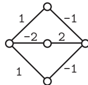
FIGURE 10. G_{n,3} consists of two even subcycles.
