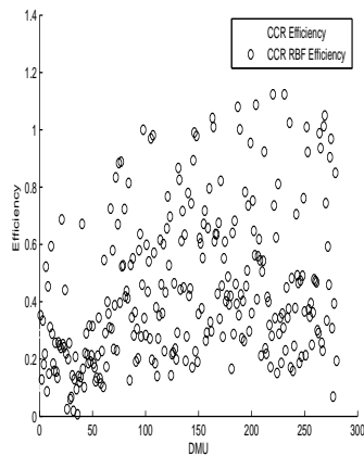
FIGURE 4. The comparison between result of CCR and CCR-RBF: the squares denote the efficiency score computed by CCR and the circles represent the efficiency score computed by CCR-RBF.
