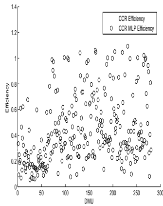
FIGURE 3. The comparison between result of CCR and CCR-MLP: the squares show the efficiency score computed by CCR and the circles represent the efficiency score computed by CCR-MLP.
