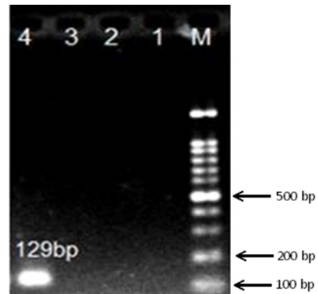
Fig. 1. The results of specificity determination of the assay. M: Marker 100 bp; 1: Negative control; 2: No amplification of Newcastle disease virus (B1 Type, LaSota Strain); 3: No amplification of Avian influenza virus (H9N2); 4: 129 bp band of IBV 5' UTR.
