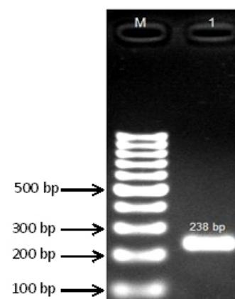
Fig. 3. The specific amplification of recombinant IPC plasmid showed 238 bp band.
