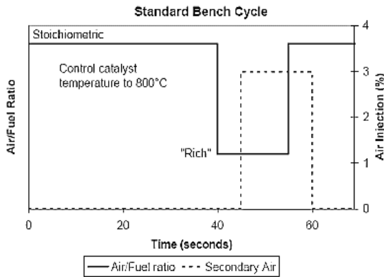
Figure 2: The Standard Bench Cycle used for accelerated aging of the catalyst [9].
