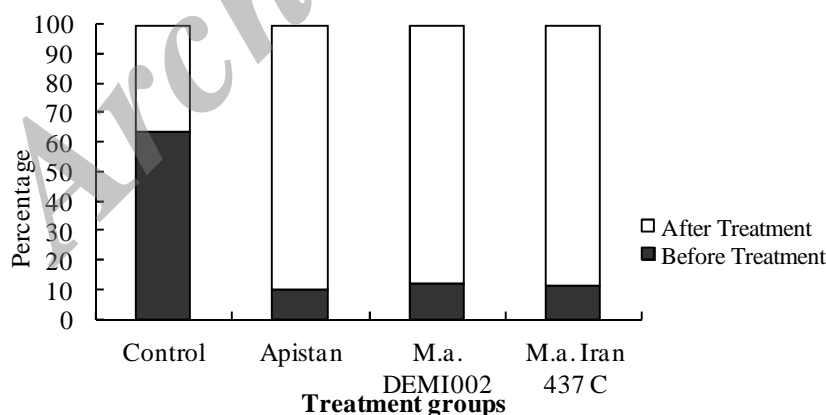
Fig. 1. The percentages of collected fallen mites before and after treatment within each group (Control: n= 40, Apistan: n= 155, Metarhizium anisopliae DEMI002: n= 170 and M. anisopliae Iran 437C: n= 74)
