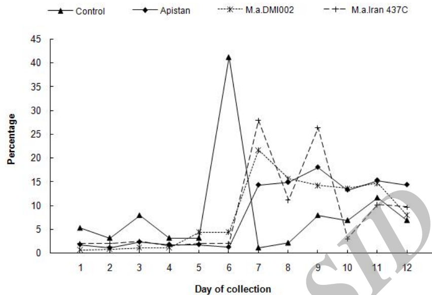
Fig. 2. Mean percentage of daily collected fallen mites from four experimental groups. (Day 6= 3 days before treatment and Day 7= day of treatment commencement)
