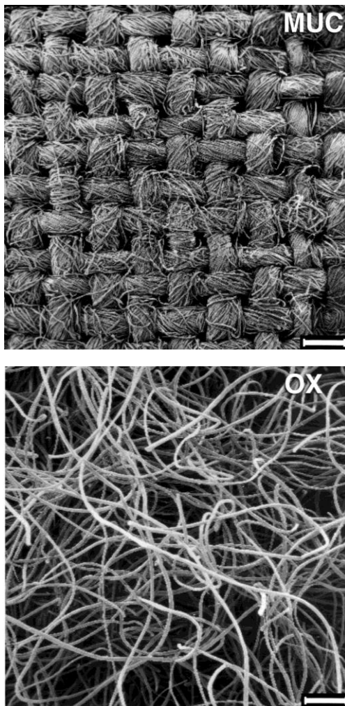
Fig. 2. Scanning electron micrographs of the Munich (MUC) and Oxford (OX) fabrics. Scale bars: 500 \mu m
