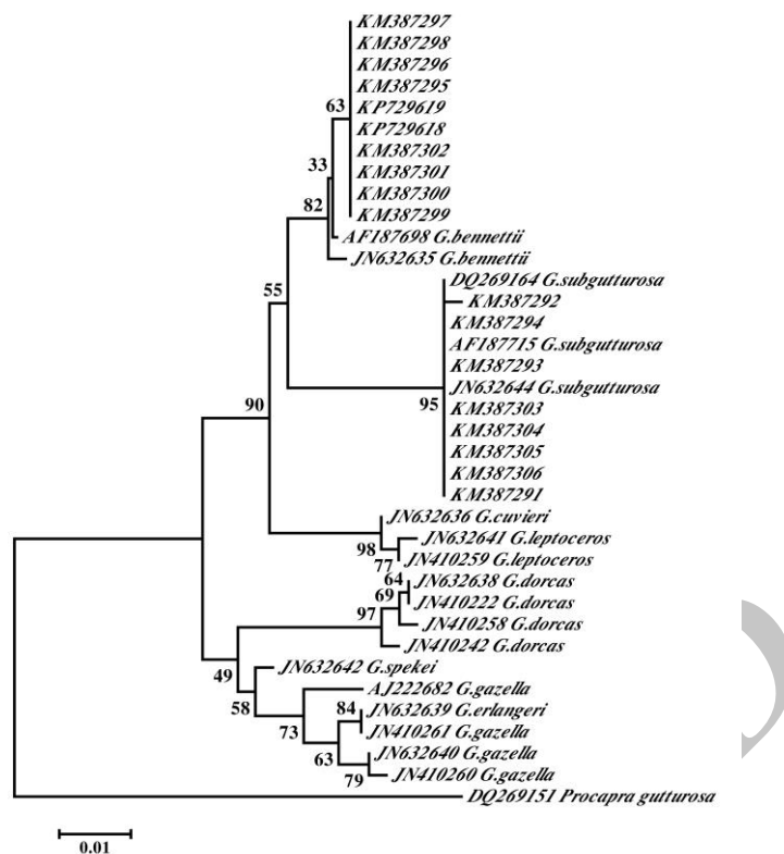
Fig. 1. Maximum Likelihood tree based on the analysis of 410 bp of Cyt-b sequences. The resulting phylogenetic tree shows Kharg and Kish Islands gazelles are Gazella subgutturosa and Hengam and Hormoz Islands gazelles are Gazella bennettii .
