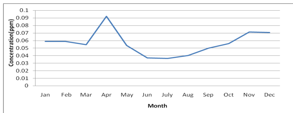
Fig. 3. Monthly variations of NO 2 concentrations in Tehran.
