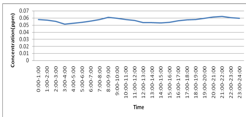
Fig. 2. Diurnal variations of NO 2 concentrations in Tehran.
