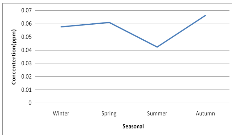
Fig. 4. Seasonal variations of NO 2 concentrations in Tehran.
