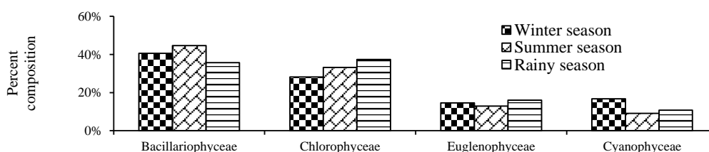
Fig. 3. Percent composition of phytoplankton in water of Turag River in three study seasons during November 2015- September 2016.
