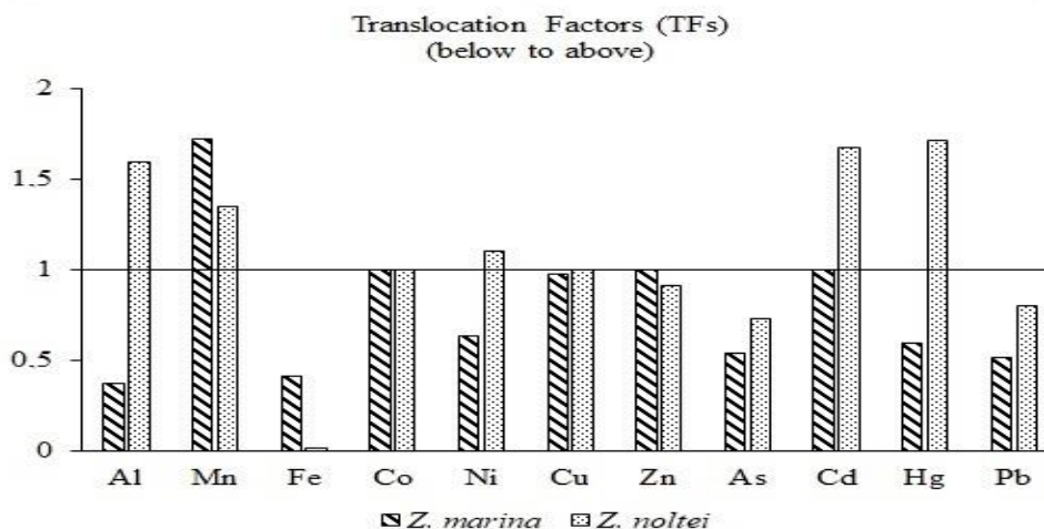
Fig. 2. Values of translocation factor ( C_{\text{leaf}}/C_{\text{root-rhizome}} ) (>1 indicate higher translocation capability)
