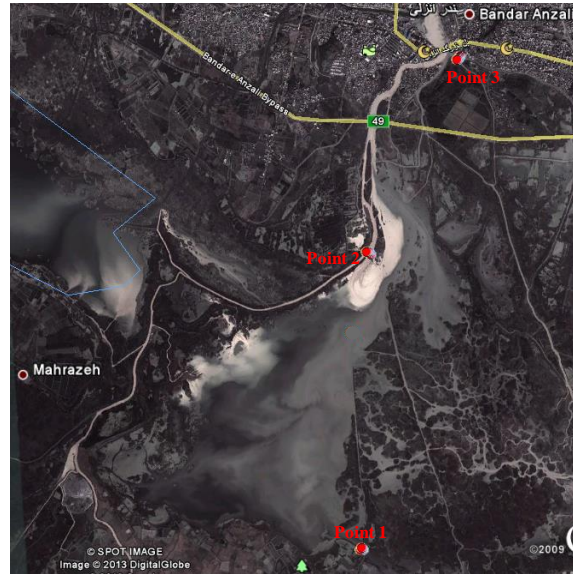
Fig. 3. Sampling points in Anzali Wetland for deriving multi variable equation.
