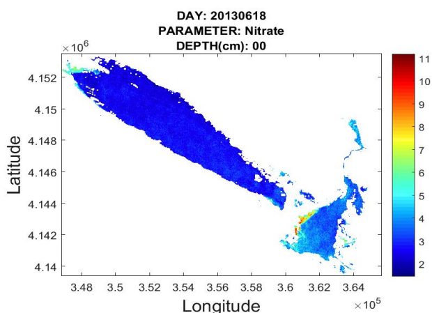
Fig. 8. Nitrate (mg L -1 ) map of surface water of Anzali Wetland using remote sensing and calibrated regression model on 18 June, 2013.
