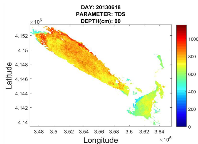
Fig. 5. TDS (mg L -1 ) map of surface water in Anzali Wetland using remote sensing and calibrated regression model on 18 June, 2013.
