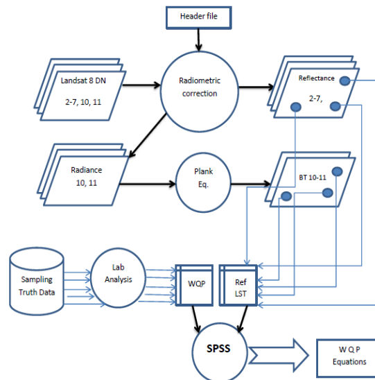
Fig. 2. Flowchart of extraction WQPs equation using remote sensing.
