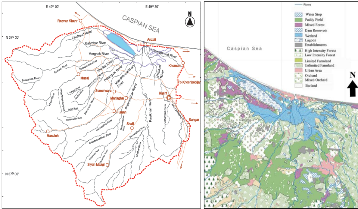
Fig. 1. Main rivers (JICA 2005) and land use (Naseh et al. 2012) of the Anzali Wetland watershed.
