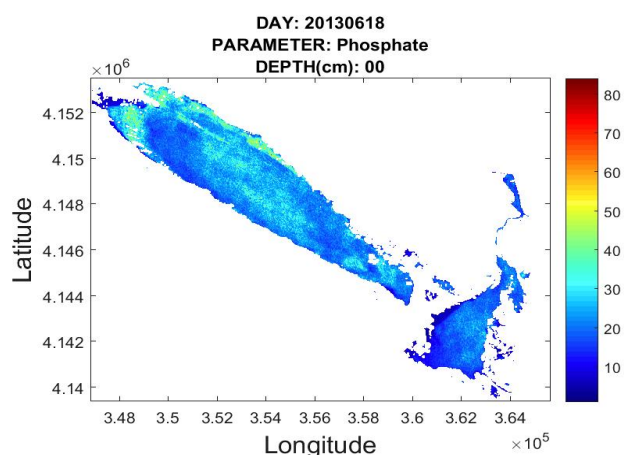
Fig. 7. TP (mg L -1 ) map of surface water of Anzali Wetland using remote sensing and calibrated regression model on 18 June, 2013.
