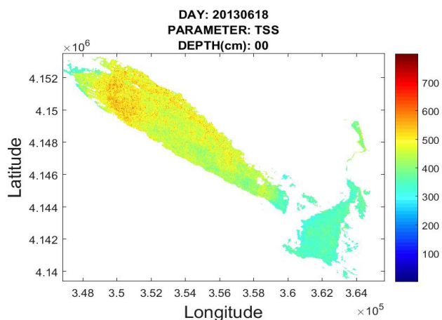
Fig. 6. TSS (mg L -1 ) map of surface water in Anzali Wetland using remote sensing and calibrated regression model on 18 June, 2013.
