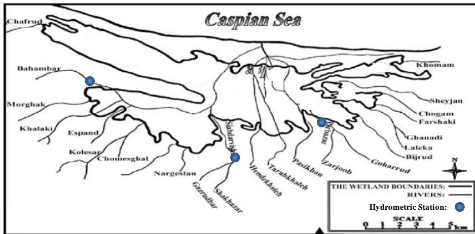
Fig. 4. Anzali Wetland, rivers leading to the wetland and hydrometric stations position.
