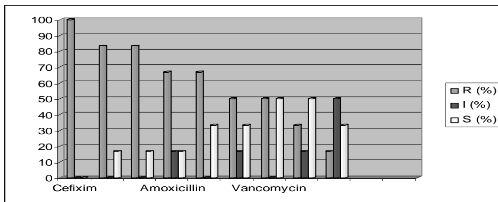
Figure 3. Gram positive microorganism sensitivity and resistance pattern to antibiotics (R: resistant, S: sensitive)
