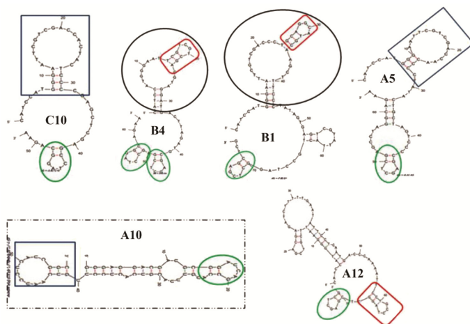
Figure 4. Secondary structure prediction. Secondary structures of five selected aptamers were predicted using mfold software. \Delta G of aptamers A12, B1, C10, A5 and B4 were -6.49, -7.85, -3.62, -5.92 and -5.03, respectively. Structure inside the box is obtained from RNA aptamer selected against extracellular domain of PSMA.
