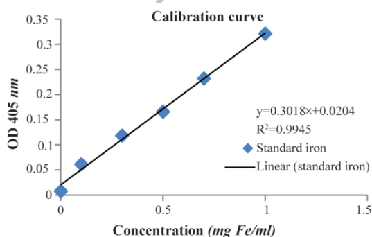
Figure 5. Standard curve of Iron standard concentration ( \mu\text{gFe/ml} ) versus absorbance at 405 nm.
