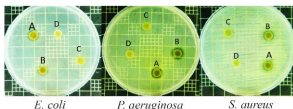
Figure 4. Antibacterial effects of pigment extract obtained from different nitrogen sources including peptone (A), yeast extract (B), (\text{NH}_4)_2\text{SO}_4 (C), and \text{NaNO}_3 (D)
