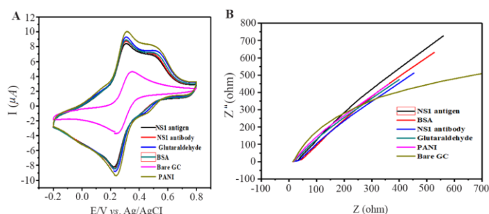
Figure 5. Behaviour of PANI modified GCE electrode (A) Cyclic voltammograms. (B) Impedance spectroscopy of different modified electrodes using 0.1 M PBS pH=7.6 containing 10 mM Fe(CN) 6 3-/4- .
