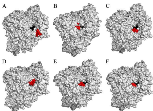
Figure 2. RNA dependent RNA polymerase (grey, surface-hydrophobicity mode) of the SARS-CoV-2 (COVID-19) in complex with different ligand drugs (red); A) MMA350 binds to the B motif; B) MMA3 binds to the F motif; C) MMA450 binds to the B and F motifs; D) IMT binds to the C and F motifs; E) BM binds to the B and F motifs; F) TF binds to the B and F motifs.
