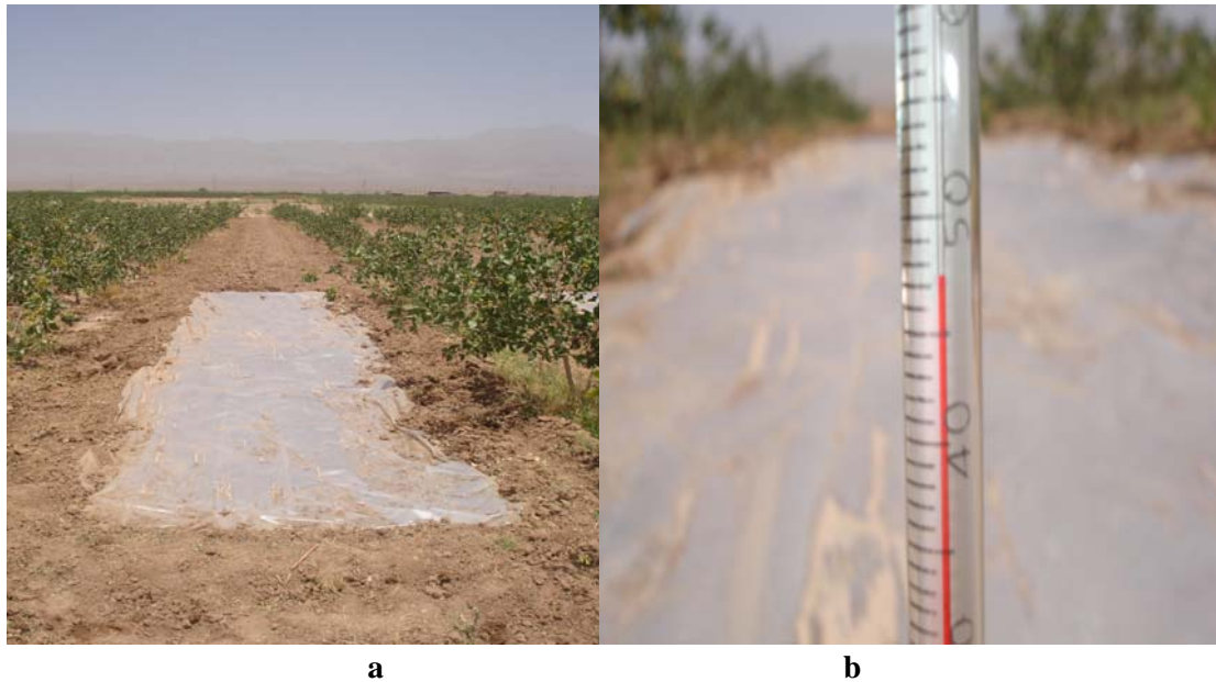
Figure 1: Application the soil solarization method by covering plastic on infected soil in pistachio orchards in Kerman (a) and increased soil temperature after covering soil (b).
