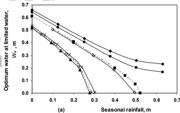
Figure 3. Relationships between optimum water and seasonal rainfall under water limiting conditions in different years after planting with different corm intensity: \blacklozenge , 1 year ( 9.5 \text{ t ha}^{-1} ); \blacksquare , 2 years ( 11.8 \text{ t ha}^{-1} ); \blacktriangle , 3 years ( 16.7 \text{ t ha}^{-1} ); \times , 4 years ( 15.8 \text{ t ha}^{-1} ); \circ , 5 years ( 16.4 \text{ t ha}^{-1} ); \bullet , 6 years ( 10.4 \text{ t ha}^{-1} ); \diamond , 7 years ( 12.0 \text{ t ha}^{-1} )
