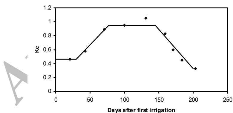
Figure 2. Crop coefficient for saffron at different growth stages.
