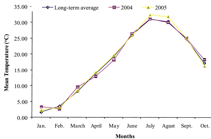
Figure 2. Long term average monthly temperature at Diyarbakir and average monthly temperature during two years.
