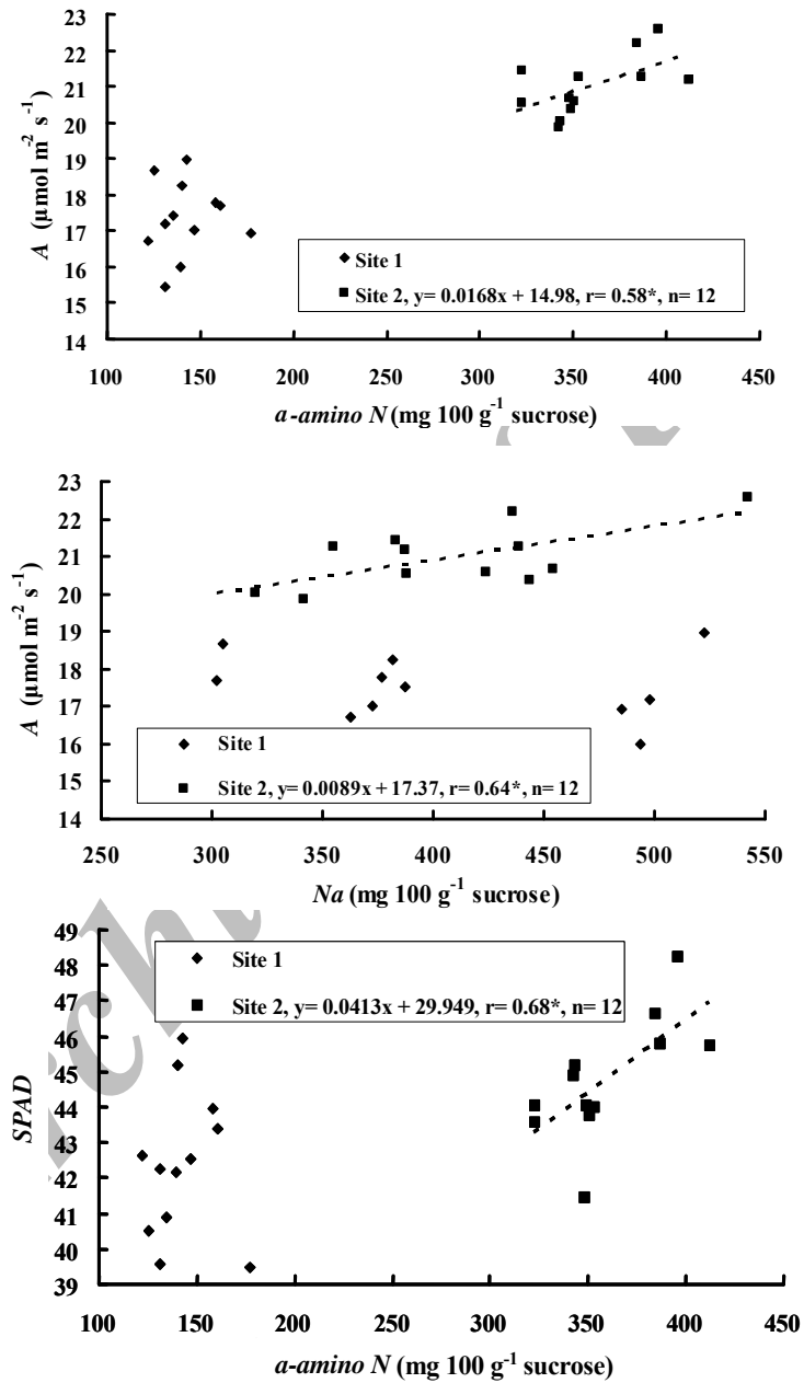
Figure 4. Relationships of root Na and \alpha\text{-amino N} concentration with A and \text{SPAD} for each site. *: P < 0.05 .
