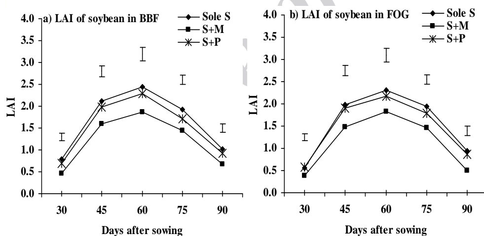
Figure 2. Leaf area index (LAI) of soybean as sole and in association with maize and pigeonpea under (a) broad-bed and furrow and (b) flat on grade; 'sole S' indicates sole soybean, 'S+M' is soybean/maize intercropping and 'S+P' soybean/ pigeonpea intercropping; vertical bars indicate LSD ( P < 0.05 ).
