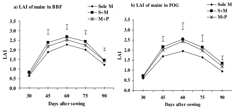
Figure 3. Leaf area index (LAI) of maize as sole and in association with soybean and pigeonpea under (a) broad-bed and furrow and (b) flat on grade; 'sole M' indicates sole maize, 'S+M' is soybean/maize intercropping and 'M+P' maize/pigeonpea intercropping; vertical bars indicate LSD ( P < 0.05 ).
