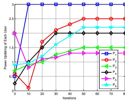
Fig. 3. The illustration of updating transmit power by users and reaching the KSBS operating point.
