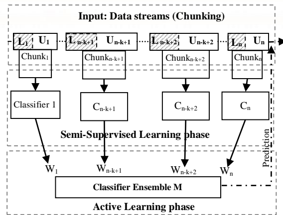
Fig. 2. A general classifier ensemble framework for learning from data streams
