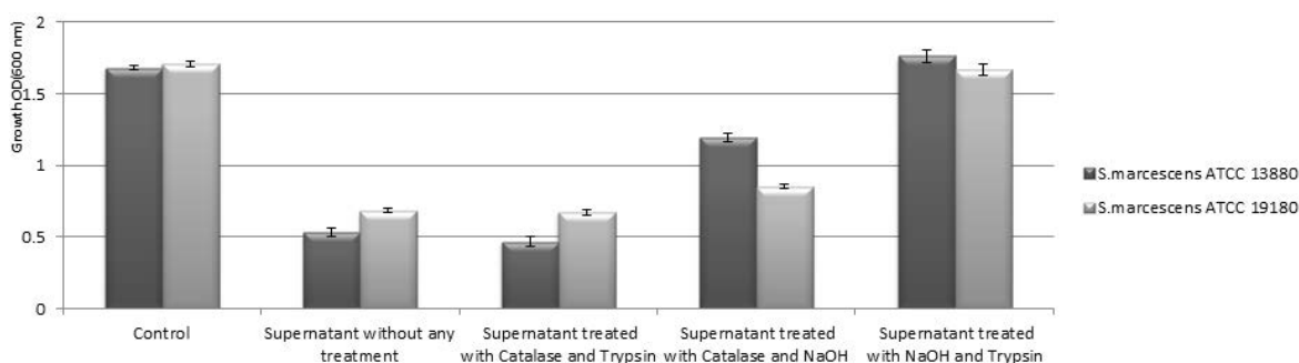
Fig. 2. MODA of cell-free supernatant from L. plantarum ATCC 8014 on S. marcescens strains growth.
