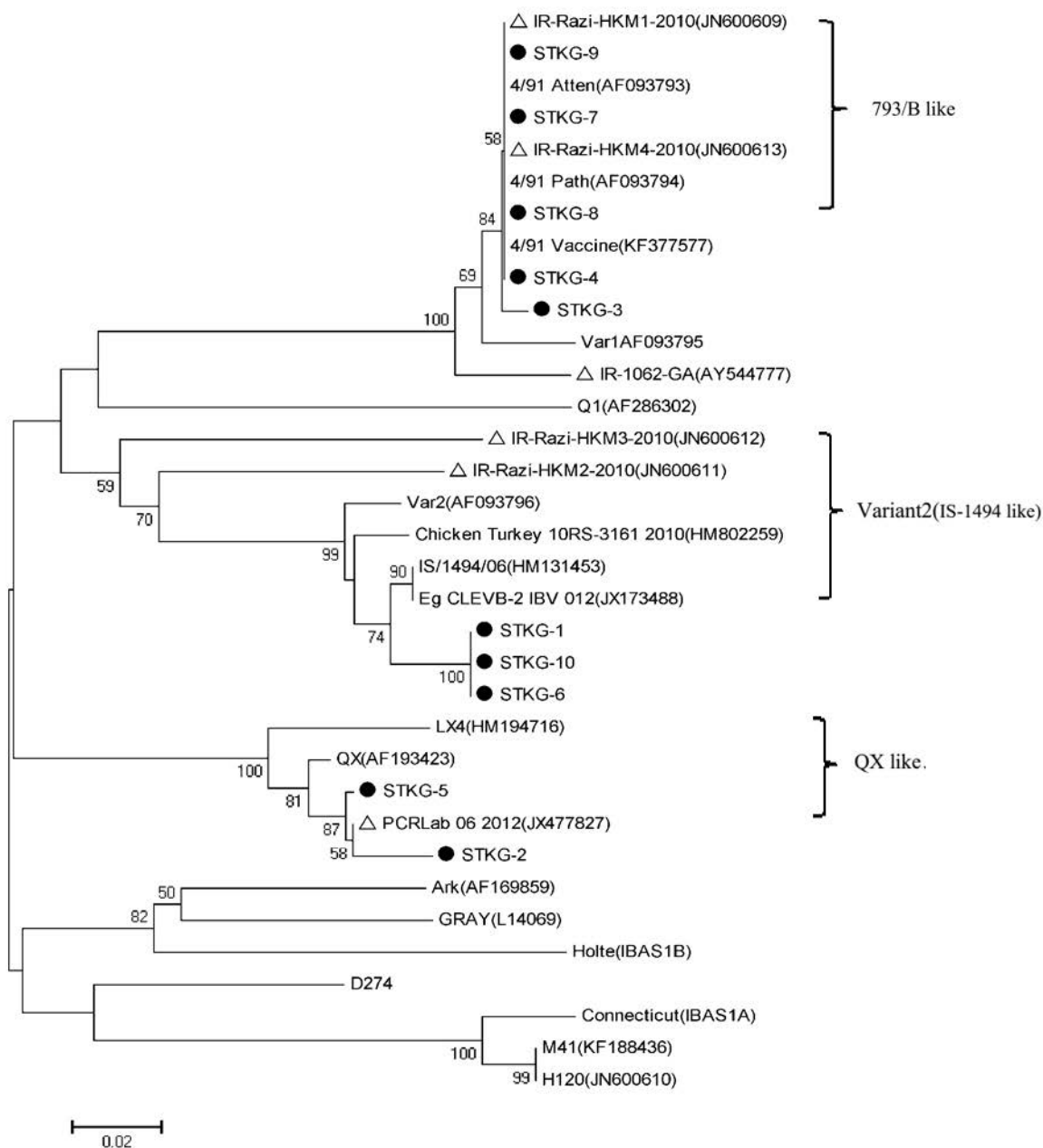
Fig. 2. Nucleic acid Phylogenetic relationships of S gene avian infectious bronchitis virus (IBV) detected from backyard chicken in Iran, 2014. The phylogenetic tree was generated using neighboring joining model with MEGA (version 5.1 beta). Numbers below branches indicate bootstrap value from 1000 replicates, bootstrap values. Horizontal distances are proportional to the minimum number of Nucleic acid differences required to join nodes. The vertical lines are for spacing branches and labels. The analysis was based on complete open reading frames of all gene segments. The scale bar represents the distance unit between sequence pairs. The virus genome characterized in this report is indicated as Black Circle. White triangle is indicated for previous Iranian IBV isolates from commercial poultry farms. The sequences obtained from Gene Bank.
