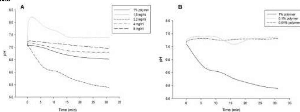
Figure 1. PH changes of BR solution following light exposure. (A) Different BR concentrations in 1% polymer (B) 3.2mg/ml BR in polymers with different w/v rate
