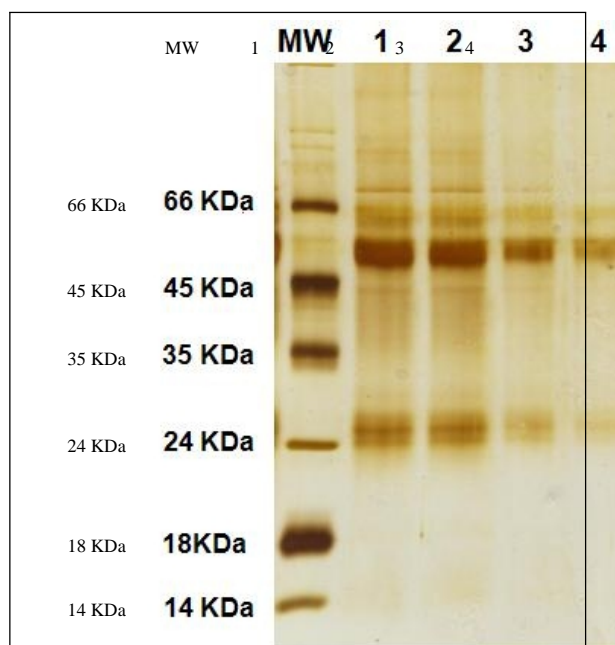
Figure 1: SDS-PAGE analysis of different concentrations of laminated layer suspension stained with silver. Lanes: 1 to 4 represent 6, 4, 2 and 1 µg LL suspension, respectively.
