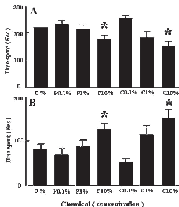
Figure 3: Effects of permethrin (P), cypermethrin (C), and vehicle (0) on the time spent by mice in the long arms (A) and short arms (B) of the EPM. Chemicals were applied topically once daily for 28 successive days. *Time spent in the long arms was shortened and the time spent in the short arms was increased by P10% and C10%, significantly ( P < 0.05 ). n = 4-10 per group
