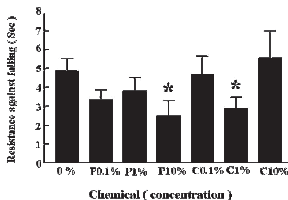
Figure 2: Effects on grasping at an inclined screen as a result of administration of various concentrations of permethrin (P) and cypermethrin (C), compared to vehicle-treated animals (0) in the mouse. Chemicals were applied topically once daily for 28 successive days. *The parameter was decreased significantly by P10% ( P = 0.044 ) and C1% ( P = 0.049 ). n = 4-10 per group
