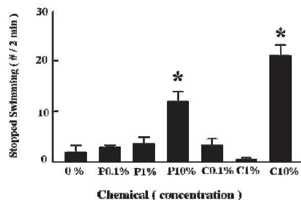
Figure 4: Despair in response to inescapable swim stress as a result of various concentrations of permethrin (P), cypermethrin (C), and vehicle (0) in the mouse. Chemicals were applied topically once daily for 28 successive days. * P10% and C10% increased despairing significantly ( P < 0.05 ). n = 4-10 per group
