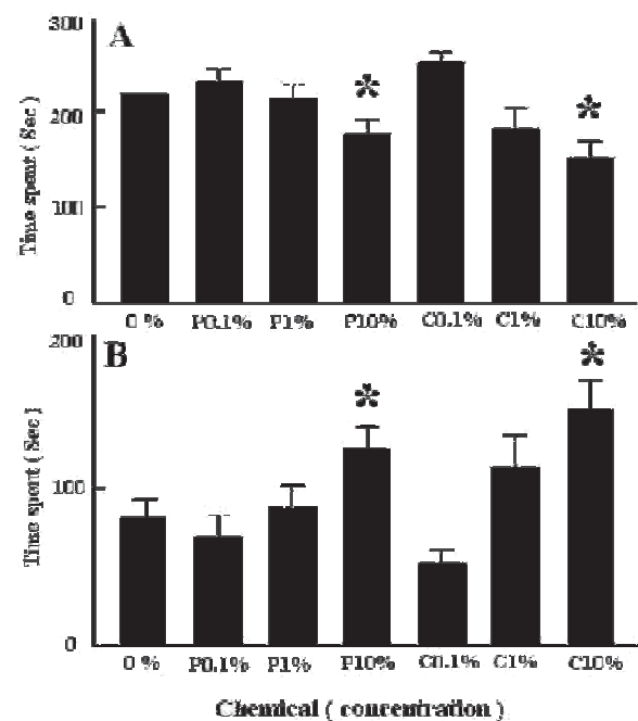
Figure 3: Effects of permethrin (P), cypermethrin (C), and vehicle (0) on the time spent by mice in the long arms (A) and short arms (B) of the EPM. Chemicals were applied topically once daily for 28 successive days. *Time spent in the long arms was shortened and the time spent in the short arms was increased by P10% and C10%, significantly ( P < 0.05 ). n = 4-10 per group
