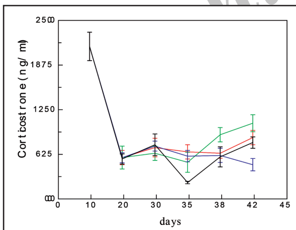
Figure 1. Effects of melatonin supplementation, darkness regime and acute heat stress on plasma corticosterone (ng/ml) concentration. ConN — ConP — Dark — Melat —
