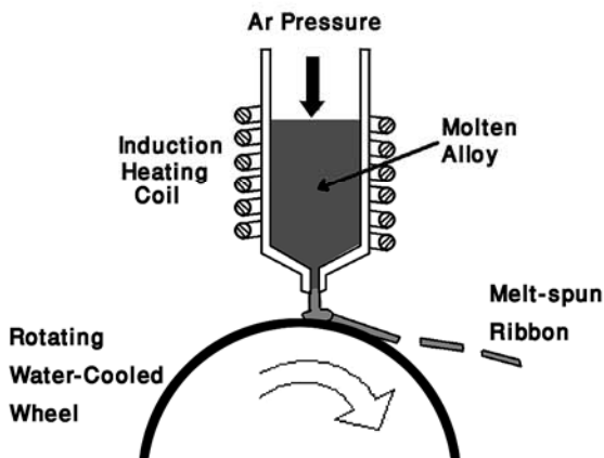
Figure 16 Melt- spinning process [16]
