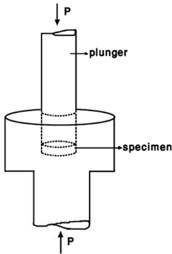
Figure 11 HPT process [11]
