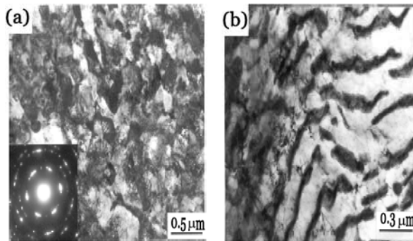
Figure 1 TEM image of a) ferrite and b) pearlite after ECAP process [5]
