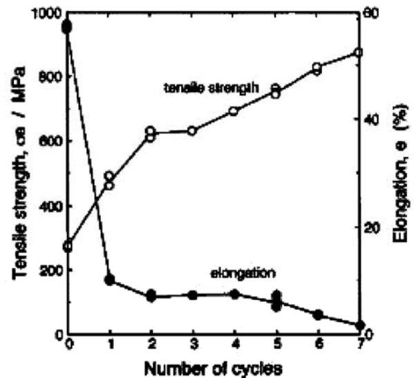
Figure 14 Mechanical properties of the alloy after different passes of ARB at 773 K [13].
