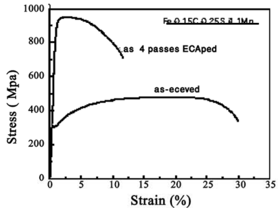
Figure 3 Stress – strain curves for the specimens before and after ECAP process [5]
