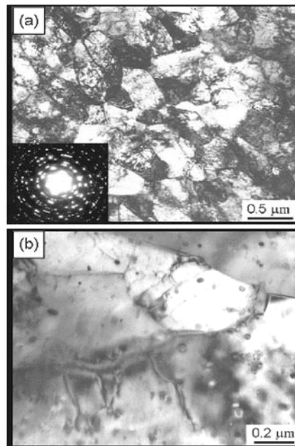
Figure 6 TEM image of a) ultra fine grain ferrite, b) nanosize vanadium carbides [8]
