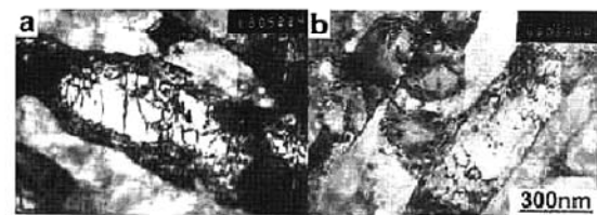
Figure 10 Microstructure of the alloy after a) 6 and b) 10 passes of ECAP process [10]
