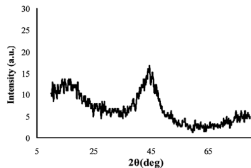
Fig 18 XRD pattern of Fe_{55}Cr_{18}Mo_7B_{16}C_4 in amorphous state.
