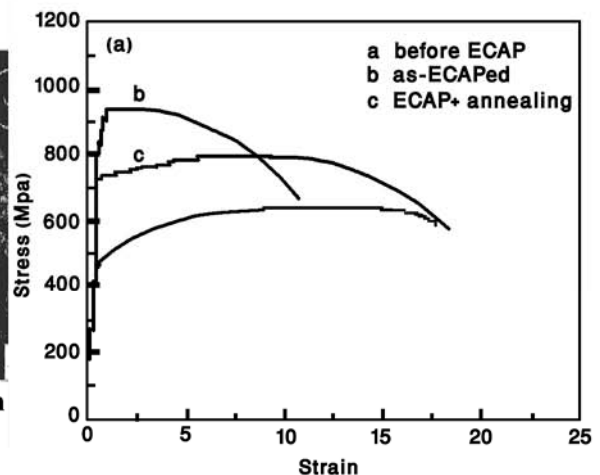
Figure 7 Stress- strain curves of vanadium alloyed steel [8]
