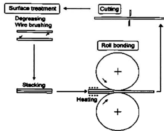
Figure 13 Accumulated roll bonding (ARB) method [13]
