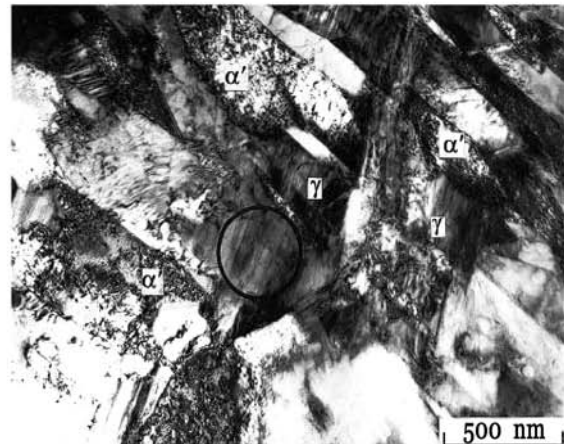
Figure 17 Microstructure of melt-spun specimens [18]
