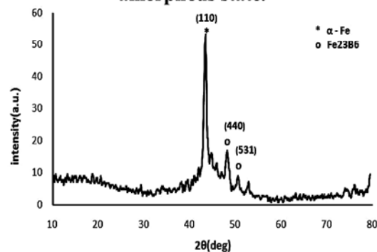
Fig 19 XRD pattern of Fe_{55}Cr_{18}Mo_7B_{16}C_4 alloy annealed at 650^{\circ}C /
