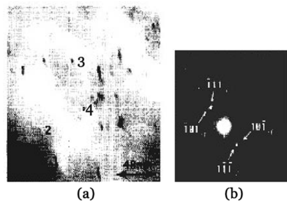
Figure 4 Bright field TEM image of nanosize martensite [6]
