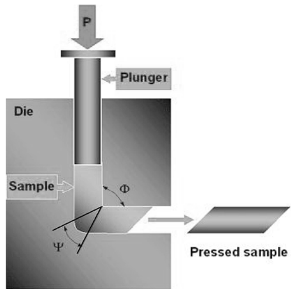
Figure 9 ECAP process
