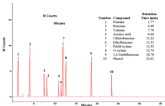
Figure 1: Chromatogram of compounds analysis with GC/MS
